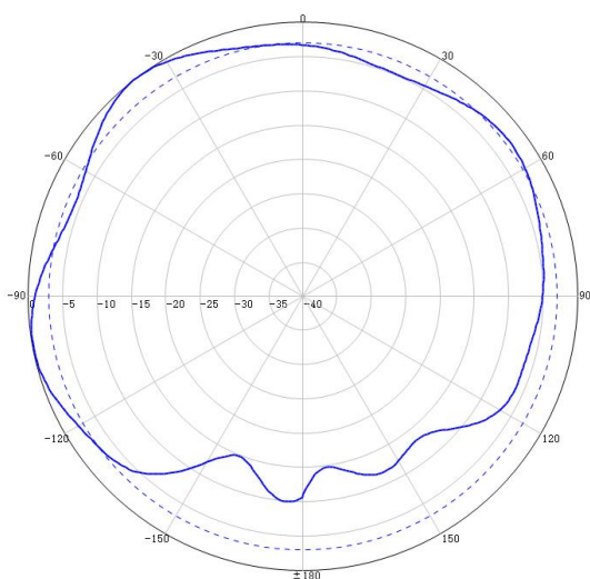
3300~4000MHz Horizontal Typical pattern:
