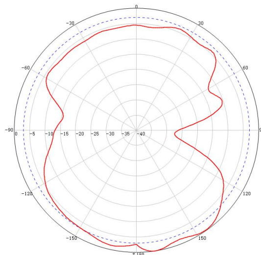
3300~4000MHz Vertical Typical pattern:
